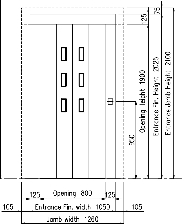
Entrance View S=1/20 (Standard Door)
