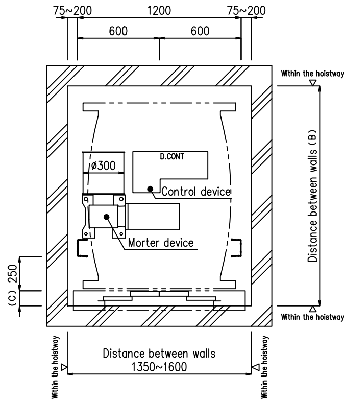
Hoistway Plan (Pit) S=1/20
