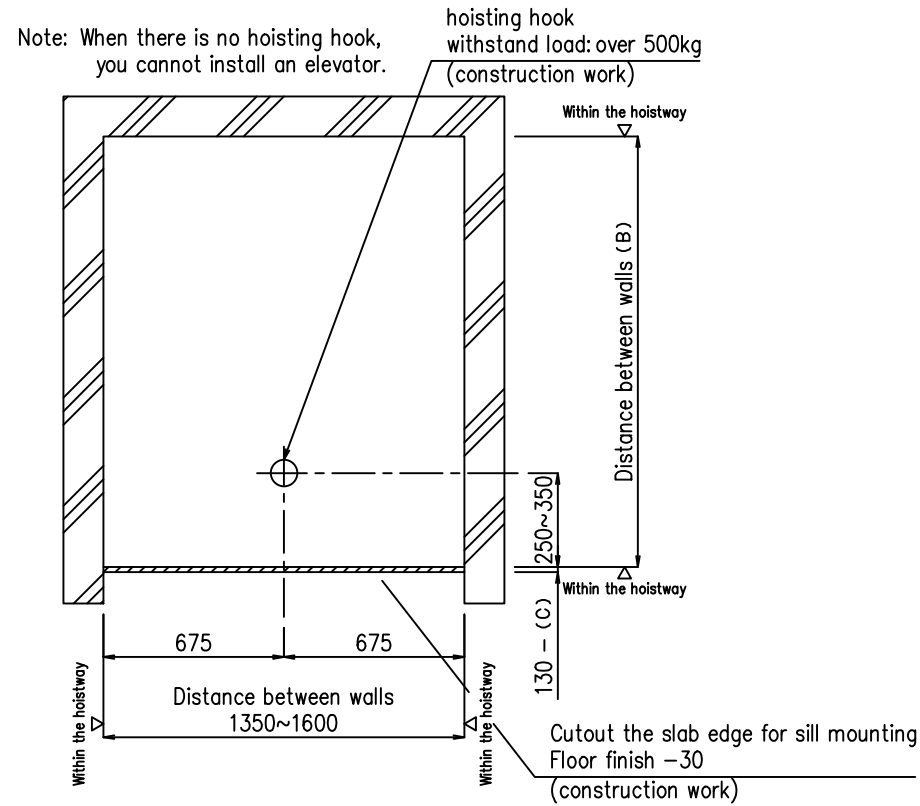
Construction Plan ( Top ) S=1/20
