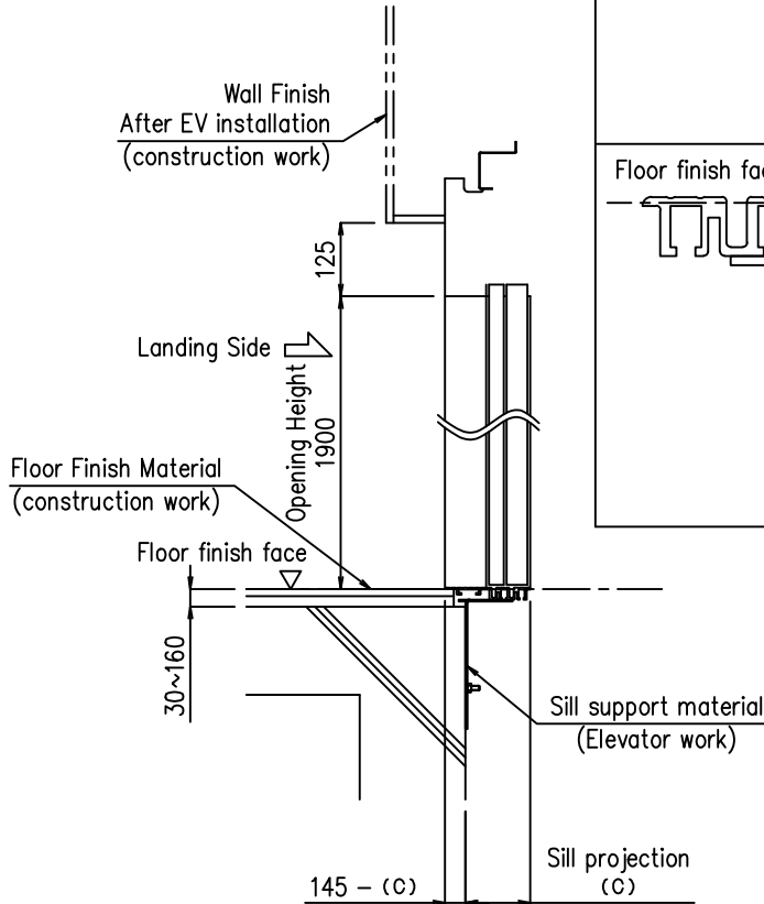
Details of Landing door S=1/10 Rear opening side
